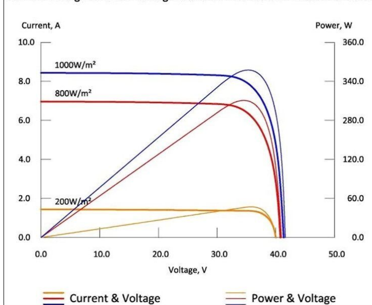
Current-Voltage & Power-Voltage characteristics various irradiance levels
